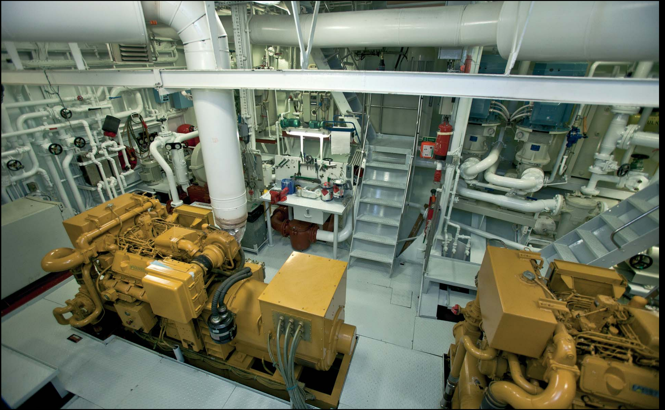
Auxiliary engine room
